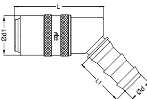
Sockets / Kupplungen
