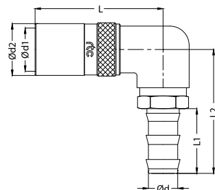
Socket / Kupplung
